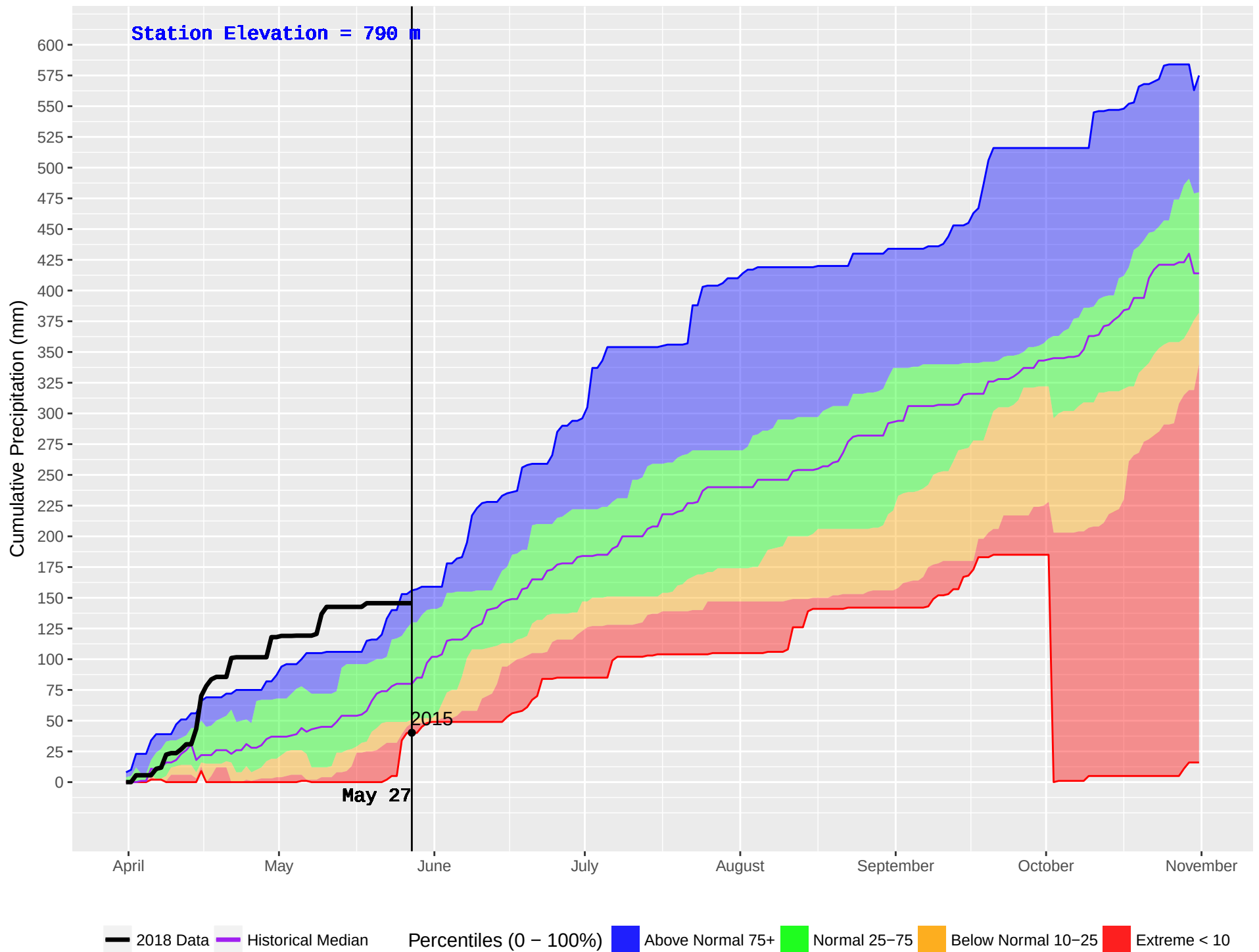
FALLS CREEK (383) : Historical (2002–2016) and Current (2018) Noon Cumulative Precipitation
