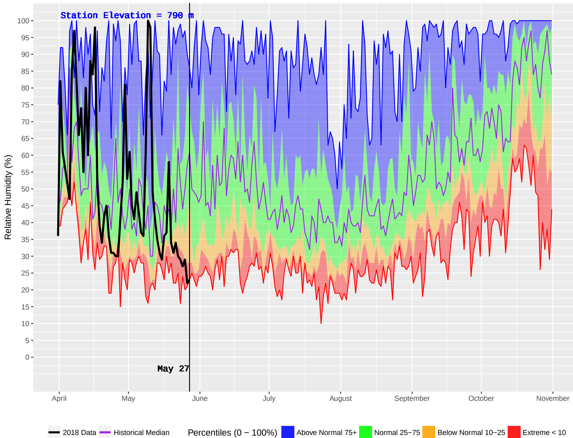
FALLS CREEK (383) : Historical (2002–2016) and Current (2018) Noon Relative Humidity
