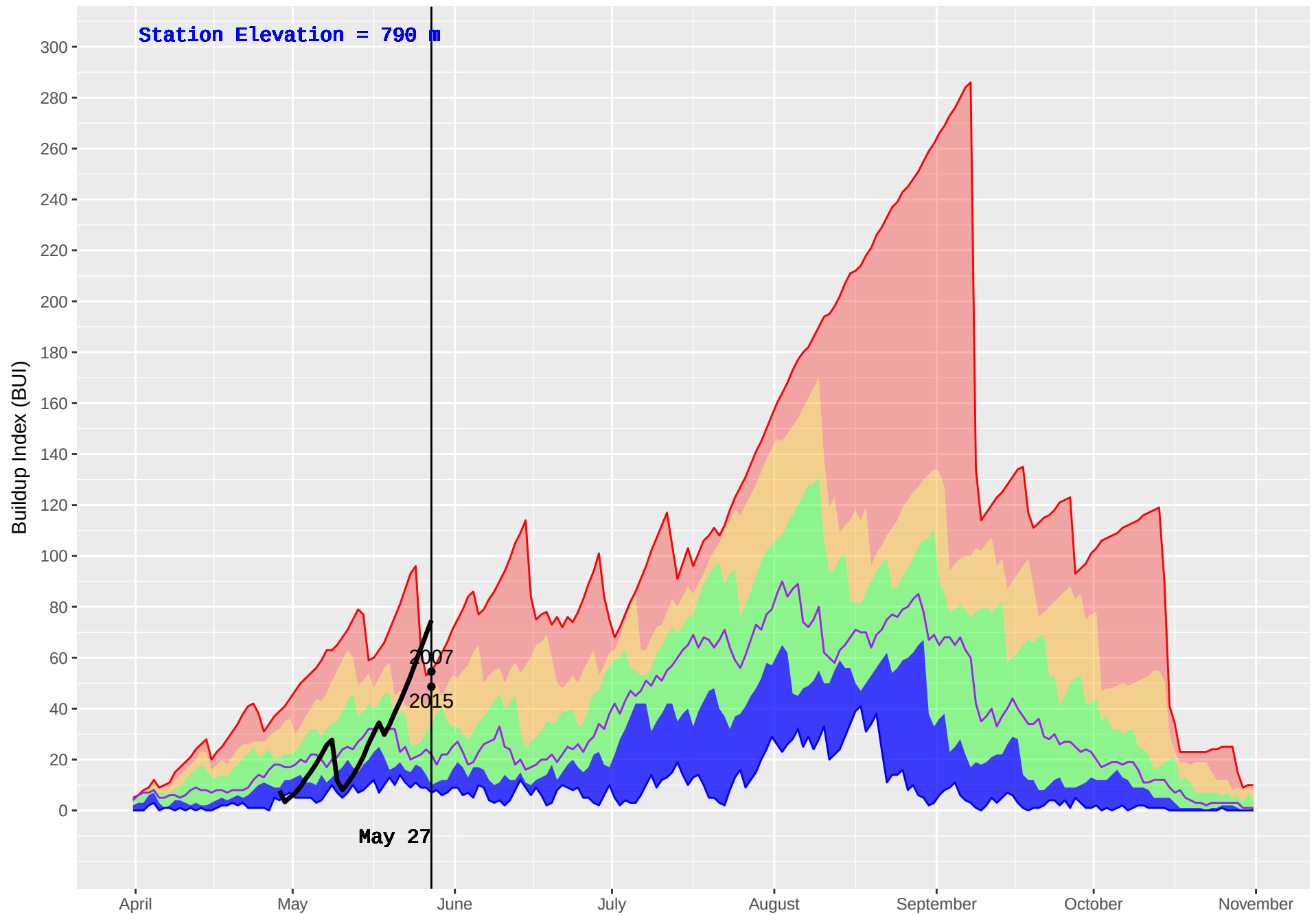
FALLS CREEK (383) : Historical (2002–2016) and Current (2018) Noon Buildup Index (BUI)
