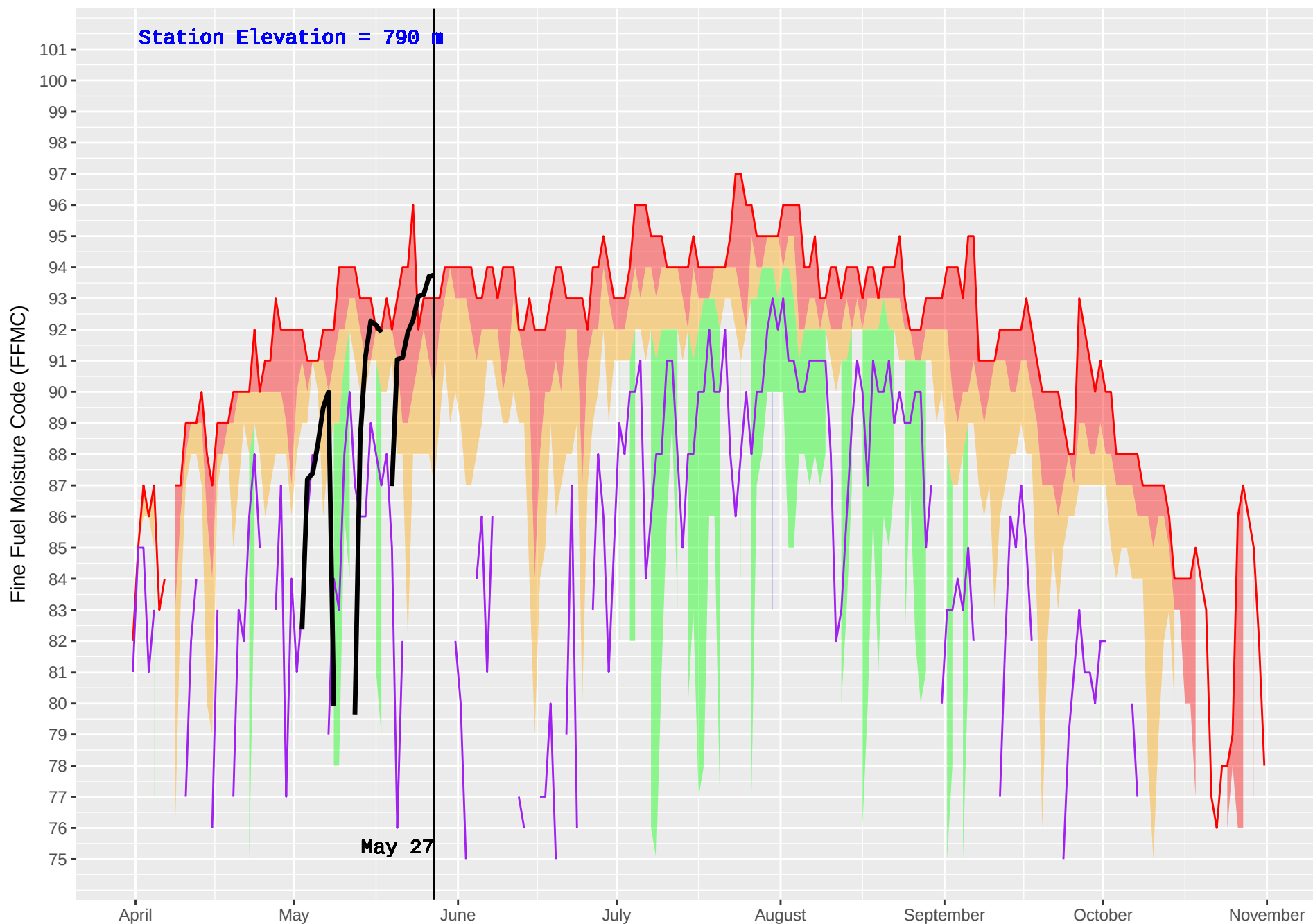
FALLS CREEK (383) : Historical (2002–2016) and Current (2018) Noon Fine Fuel Moisture Code (FFMC)
